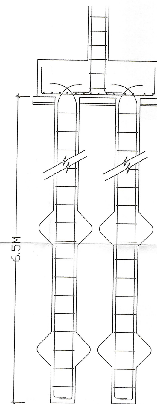
FOUNDATION DETAIL DESIGNED AS PER I.S. CODES
