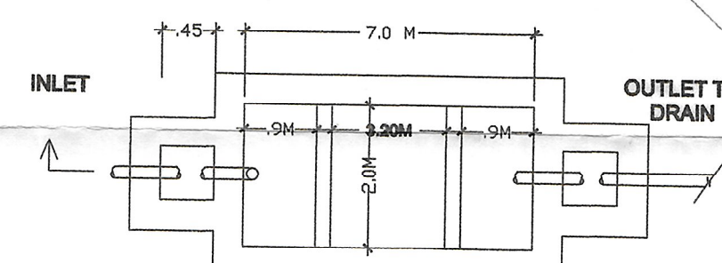
PLAN SEPTIC TANK DETAILS
